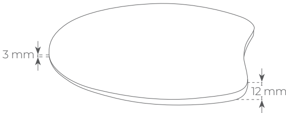
WEDGE IN TWO DEGREES FROM 12 TO 3 MM
